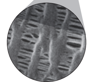
Hydrophobic membrane with pores approx. 0.03 μm
