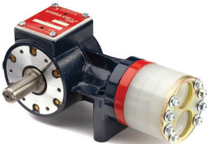
G21 external shaft-driven with Polypropylene pump head.
