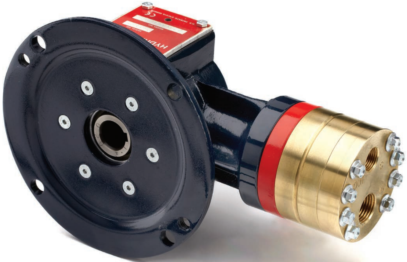
G20 close-coupled (hollow shaft) for 56C frame motors, shown with Brass pump head.
