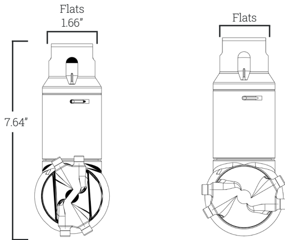
Vertical Nozzle Head Alignment Horizontal Nozzle Head Alignment Clearance Diameter: 3.35" Clearance Diameter: 3.94"
